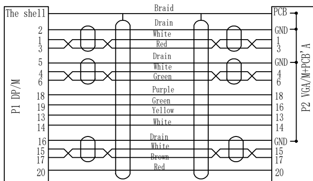
DP/M line clip drawing
