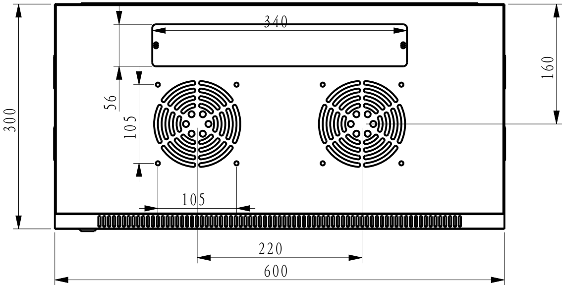
Top View
