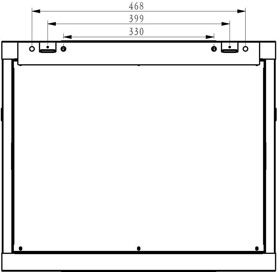
Rear View
